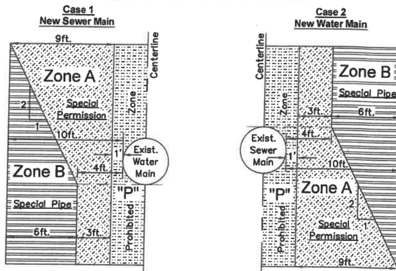
Figure 1 Parallel Construction
