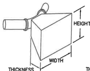
TYPICAL THRUST BLOCK CAST IRON BEND
