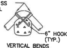
VERTICAL BENDS
