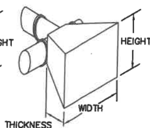
TYPICAL THRUST BLOCK TEE OUTLET
