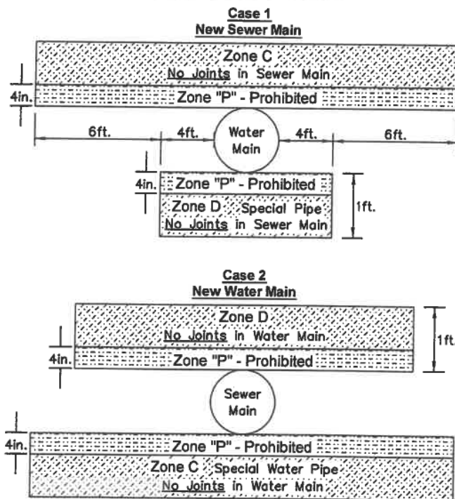
Figure 2 - Crossings
