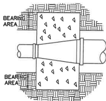
TYPICAL THRUST BLOCK REDUCER
