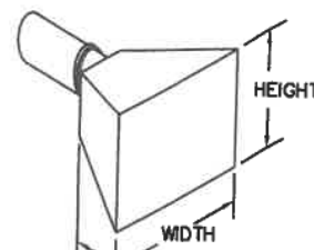
TYPICAL THRUST BLOCK DEAD END OF PIPE OR BLIND FLANGED END OF FITTINGS
